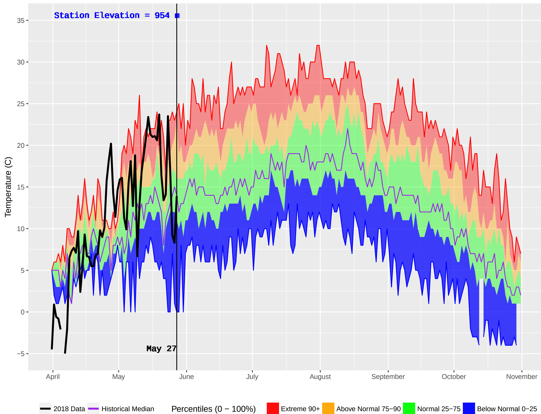
NADINA (179) : Historical (1985–2016) and Current (2018) Noon Temperature
